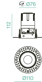
LED Module 12W-15W
