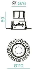
LED Module 9W
